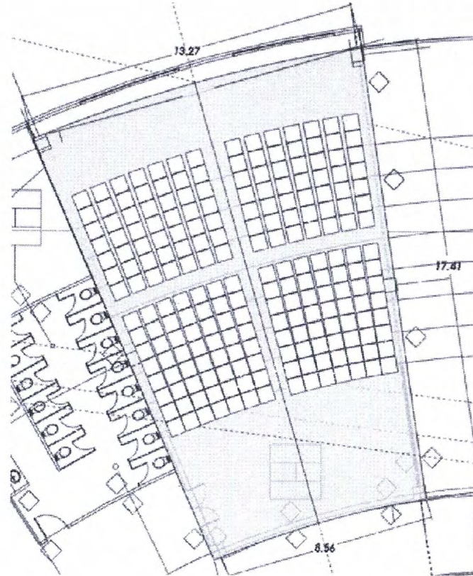
CEILING PLAN
