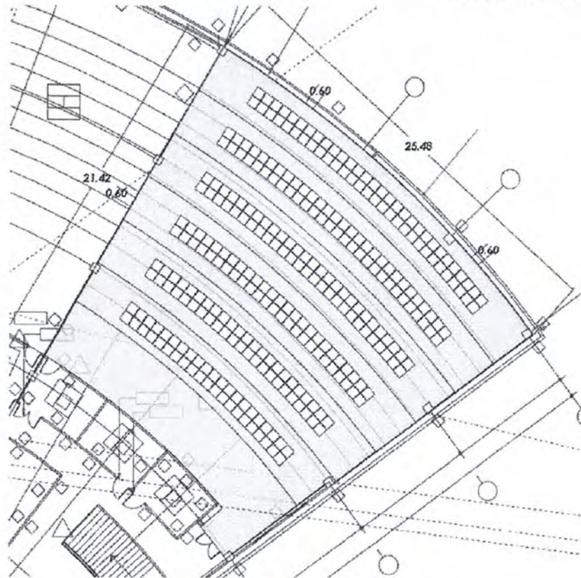
CEILING PLAN
